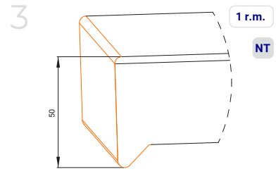
Drop nose
